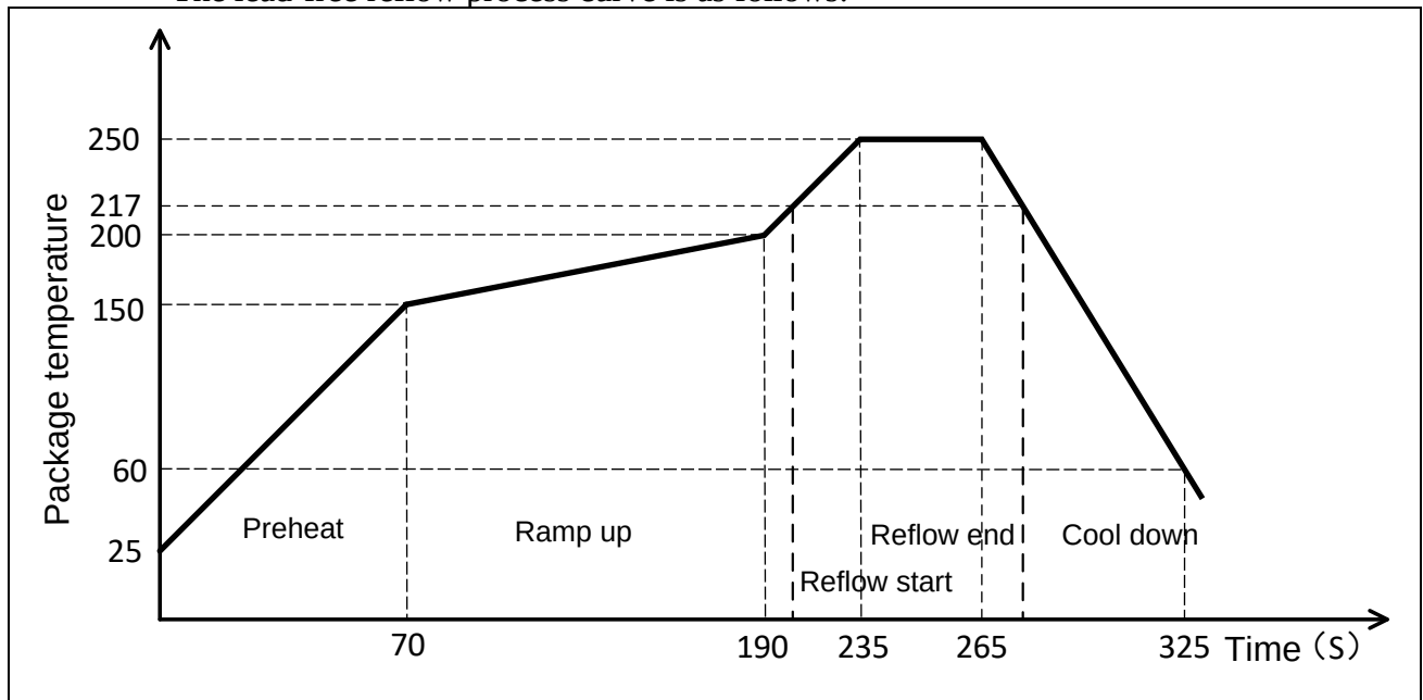
Figure 15-1 Reflow process curve
